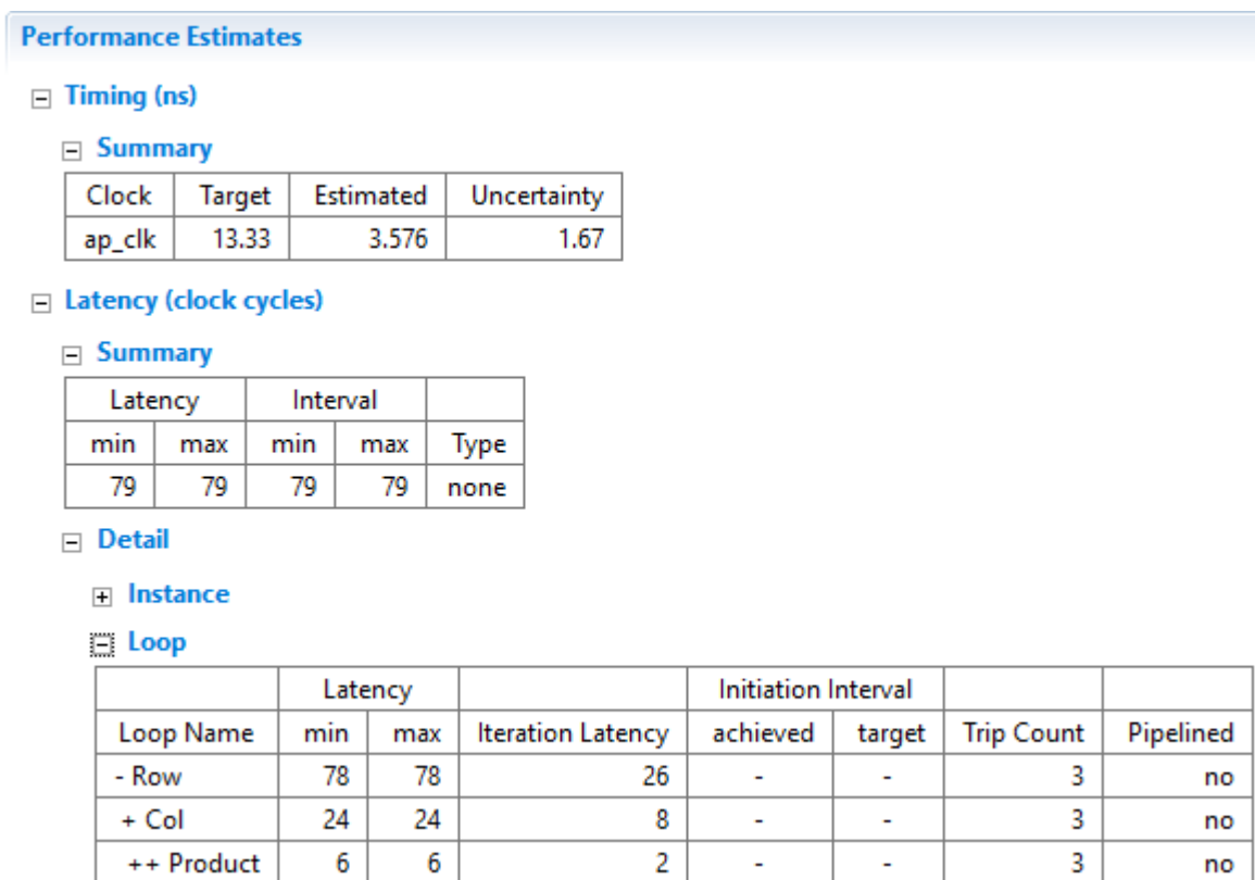
Figure 7-4: Synthesis Report for the Matrix Multiplier
