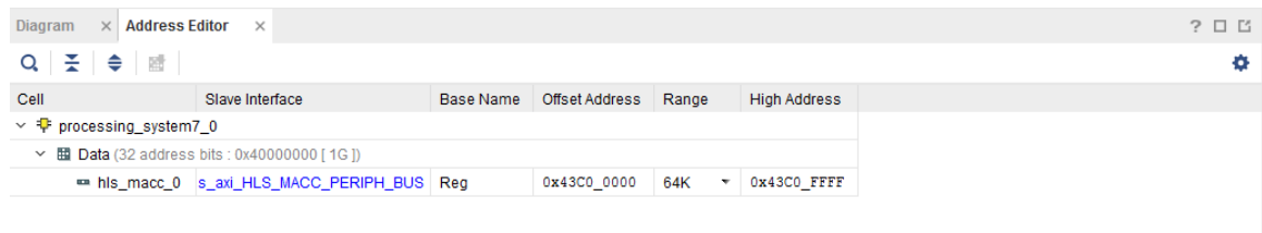
Figure 10-18: Address Editor
